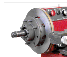
Standard Size Rotor
